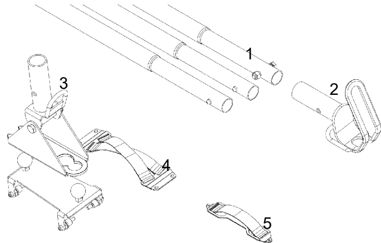
Fig. 6-3 Componenten crawler-inzettool.
