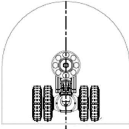
Fig. 4-5: An illustration of the C356 with the 'double-large-wheel' configuration for added surface area and grip
