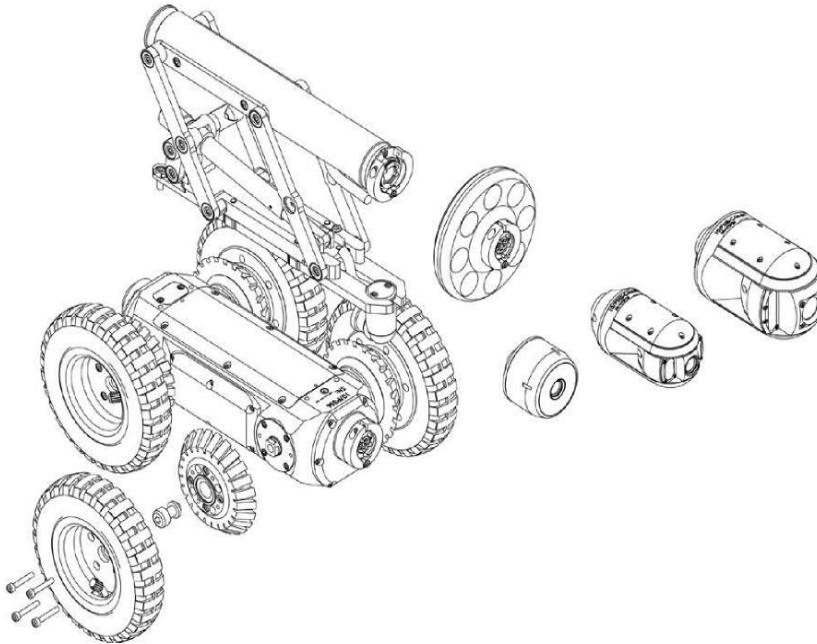
Fig. 4-1: C356 crawler assembly, showing some of the options available
