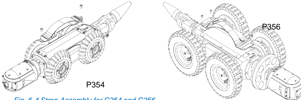
Fig. 6-4 Strap Assembly for C354 and C356.
