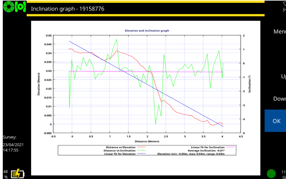
Fig. 6-26 Inclination graph.
