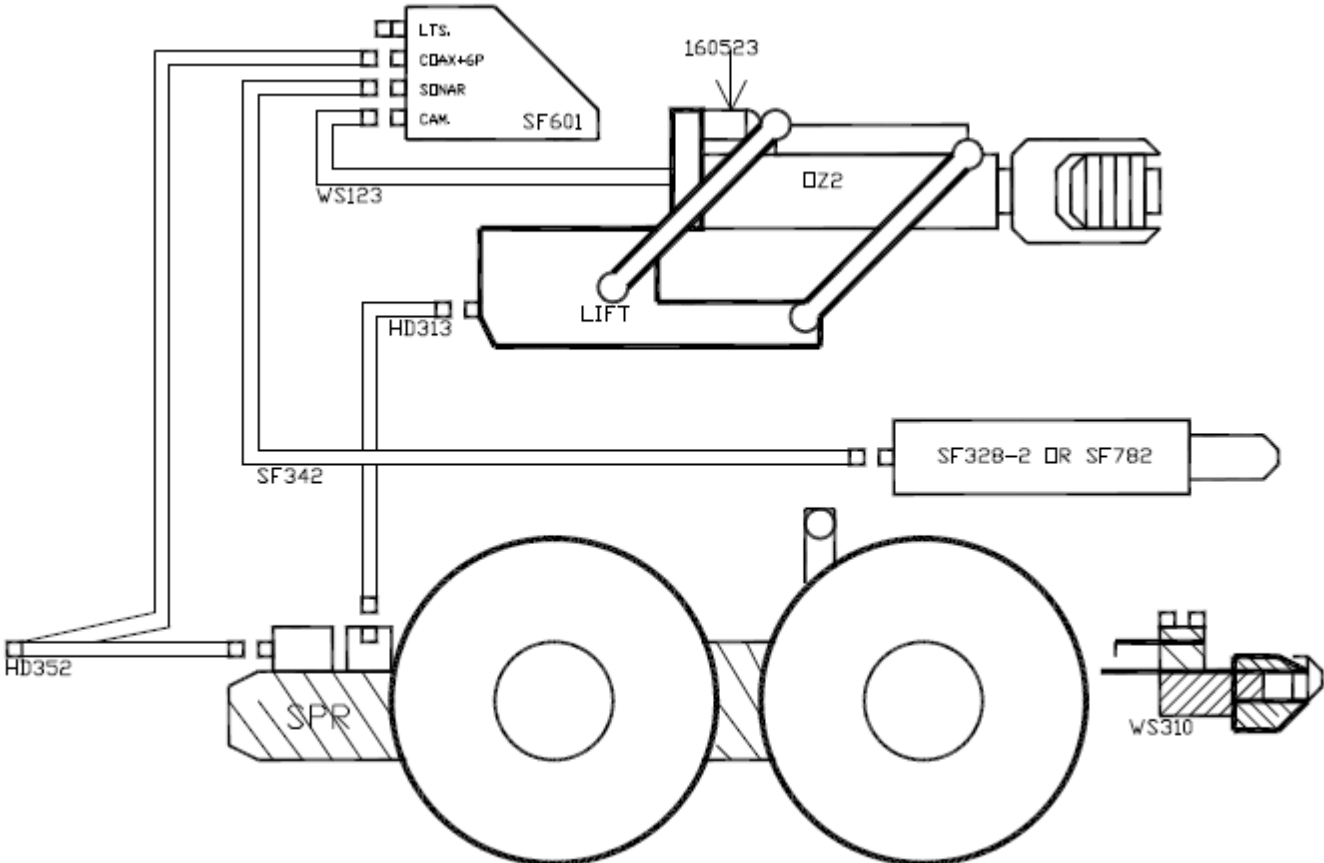
CABLING DIAGRAM
