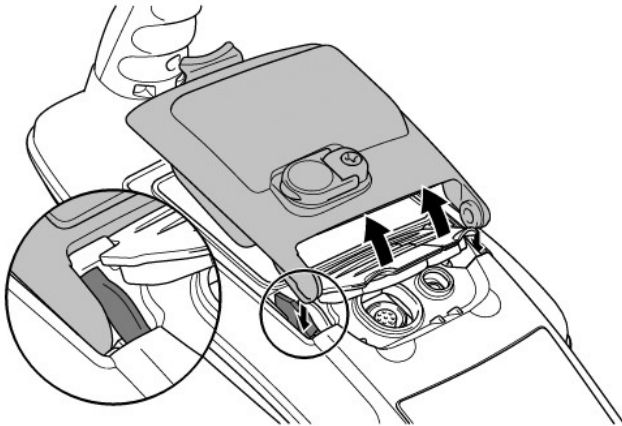
Figure 4.5: Installing a new battery pack
