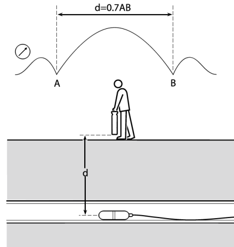
Figure 5.5 - Verifying a depth measurement
