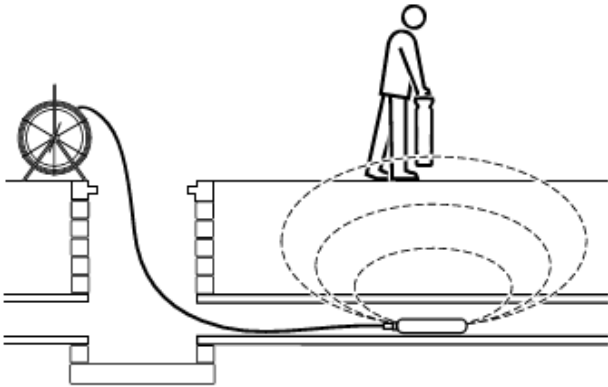
Figure 5.1 Sonde deployment
