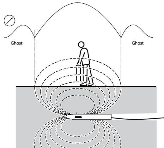
Figure 5.2 Locating a sonde
