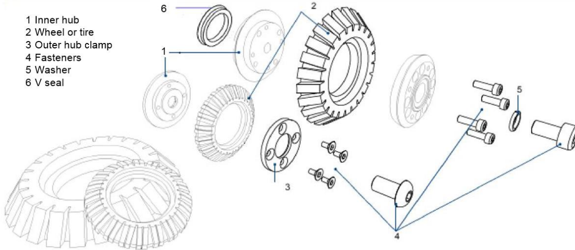
Fig. 4.2: Connecting various tires (top) and the abrasive wheels (below)
