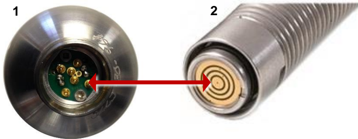
Fig. 4.24: Camera connector (1) attaches to the rod termination socket (2)
