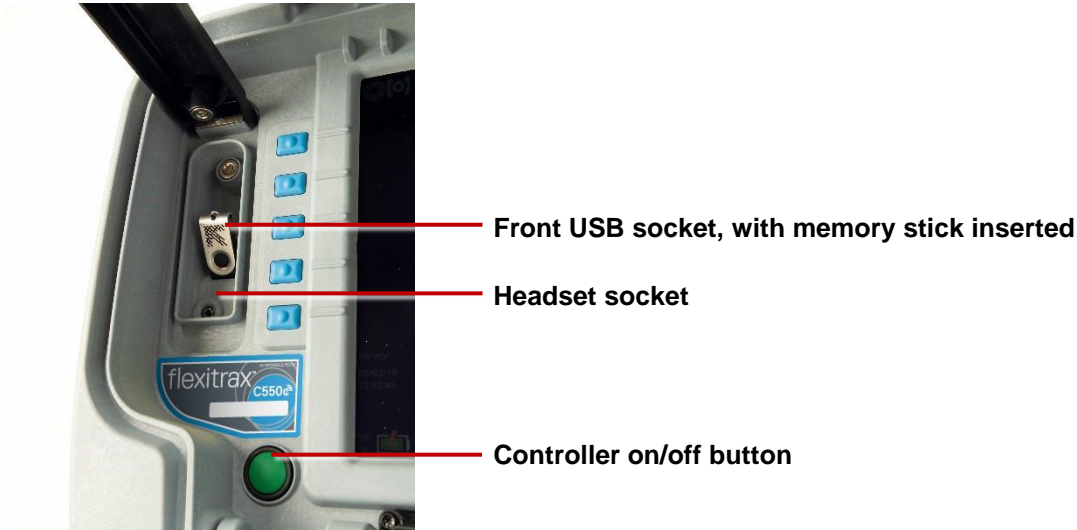
Fig. 4.21: C550c on/off button and front connections, showing headset socket and installed USB memory stick
