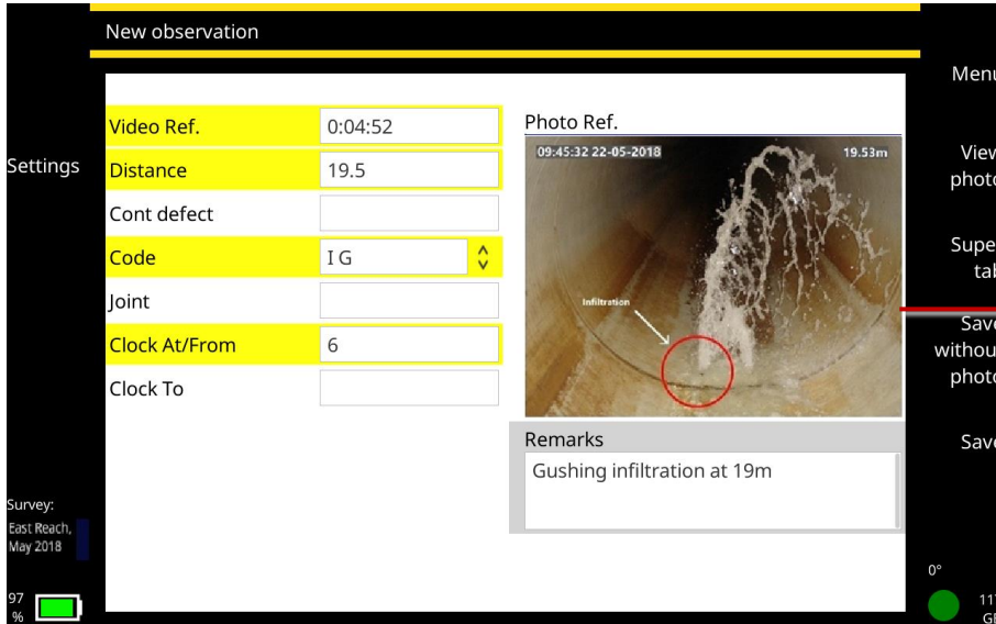
Fig. 6.27: New Observation screen showing new photo (1).
