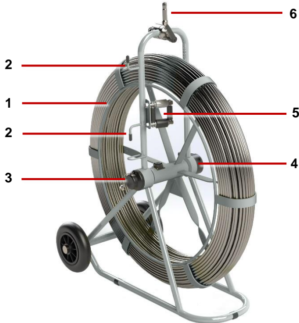
Fig. 3.12: Reel features This example shows a 543 reel.
