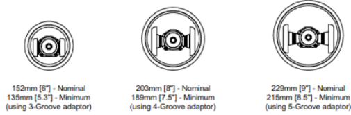
P554 Crawler (adjustable elevator) configurations (6" / 152mm to 9" / 229mm pipe)
