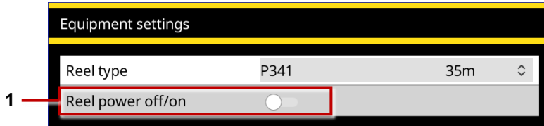
Fig. 6.28: Equipment settings. 1 Reel power off/on slider (shown in the Off position).
