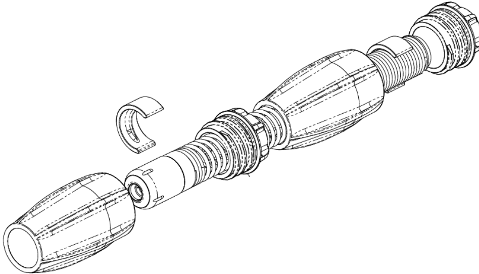
Fig. 4.29: Universal skid set for 1" (25mm) camera and flexisonde
