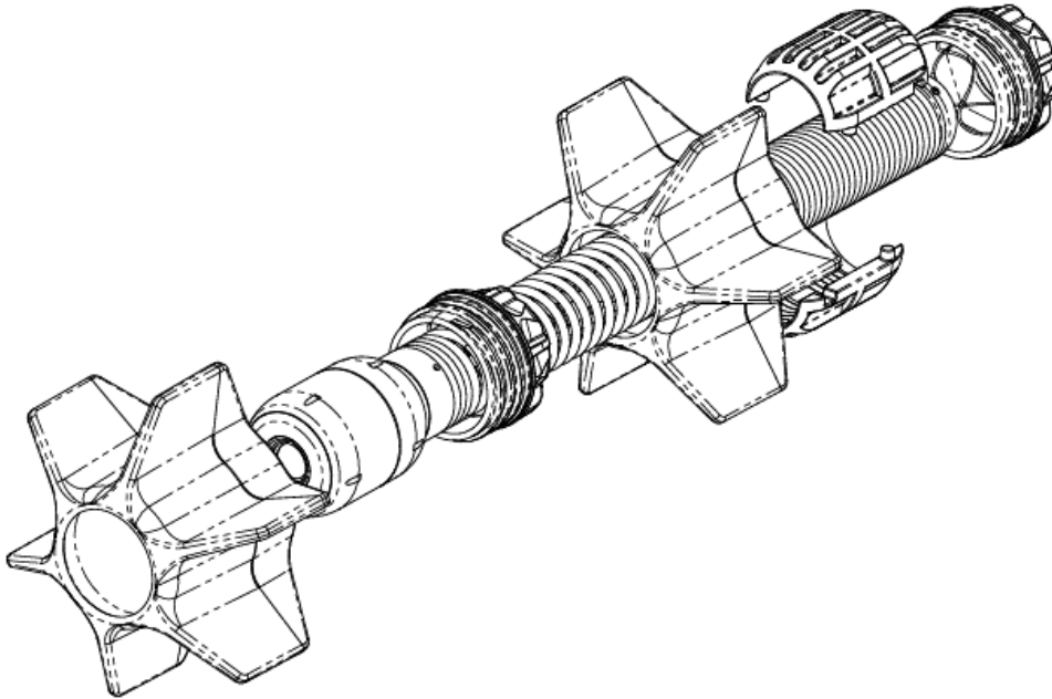
Fig. 4.30: Universal skid set for 2" (50mm) camera and 1.4" (36mm) flexisonde
