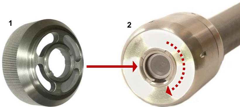
Fig. 4.25 Camera focus tool. Attach the focus tool (1) to the camera's focusing ring (2) and rotate to adjust the camera focus.
