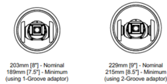
P556 Crawler rasp wheel configurations (8" / 203mm to 9" / 229mm pipe)
